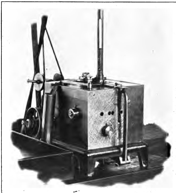
Fig. 49.—Self-Feeding Automatic Compressor for Balance Brass.
