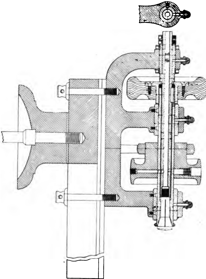
Fig. 2.—Three-Bearing, Slide Spindle Lathe.
