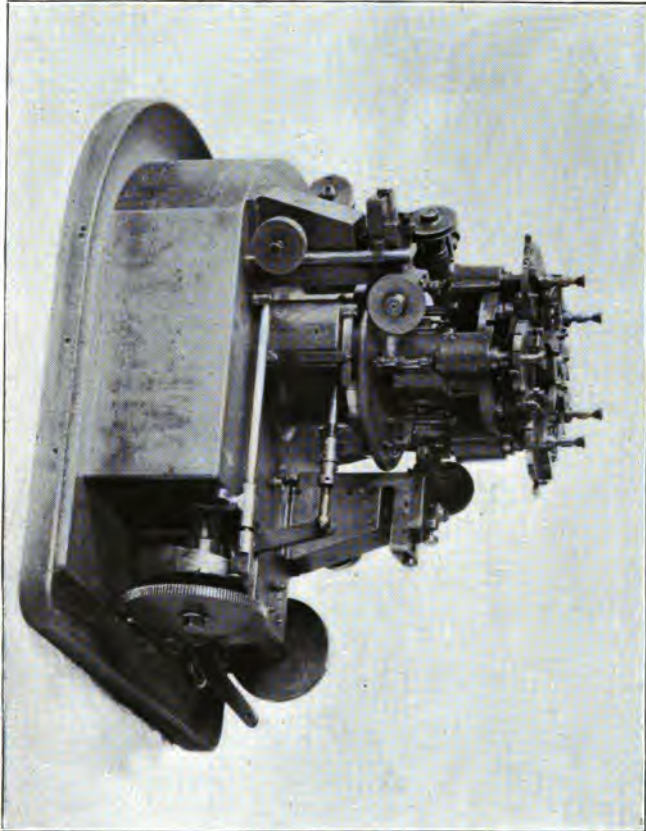
Fig. 10.—Revolving Cannon Pinion Cutter.
