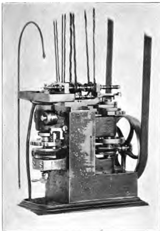
Fig. 55.—Woerd's Automatic Balance Drilling Machine.
