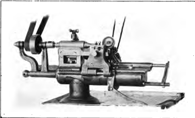
Fig. 57.—Finish Turning and Glossing Machine.
