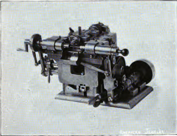
Fig. 18.—Improved Pinion Cutter.
