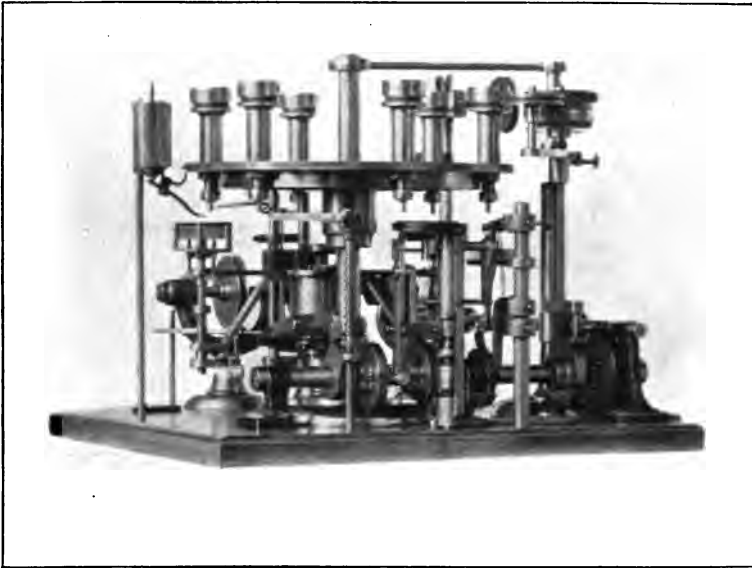
Fig. 46.—The Wood Machine for Finishing the Heads of Jewel Setting Screws.
