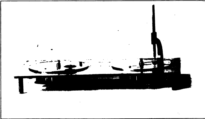
Fig. 64.—Logan Device for Testing Balances and Springs.
