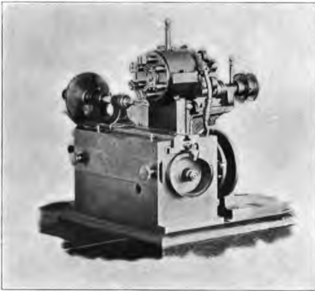
Fig. 31.—Marsh Escape Wheel Tooth Cutter.
