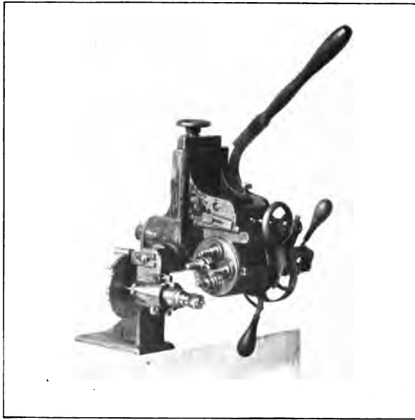
Fig. 28.—Old Escape Wheel Cutter.
