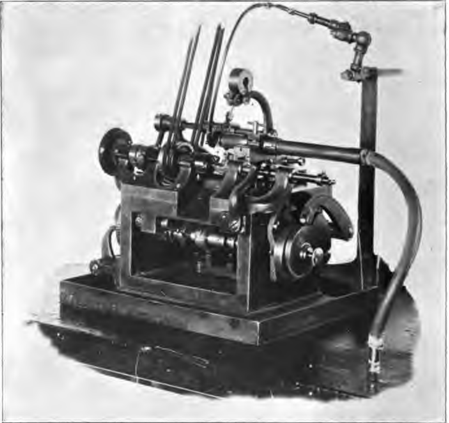
Fig. 51.—The Church Automatic Facing and Recessing Machine.
