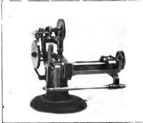
Fig. 47—Early Machine for Hammering Balance Brass.
